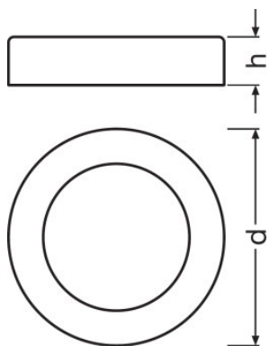
LED SURFACE ROUND 13 W 3000 K GY, LED SURFACE ROUND 13 W 3000 K WT
