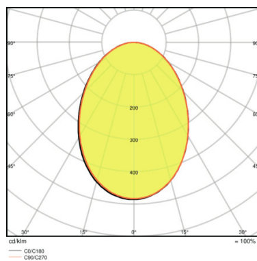
LED SURFACE ROUND 13 W 3000 K GY
