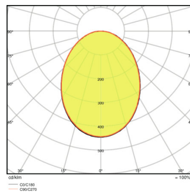
LED SURFACE ROUND 13 W 3000 K WT
