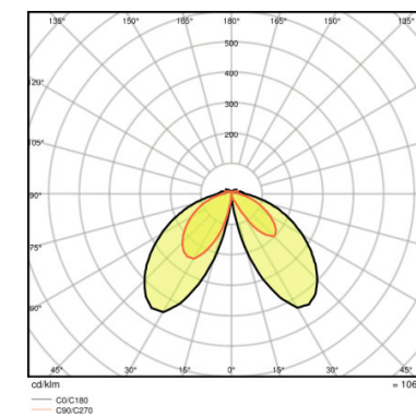
LED BOLLARD 900 LANTERN 12 W 3000 K GY
