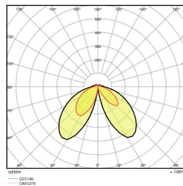
LED BOLLARD 500 LANTERN 12 W 3000 K GY
