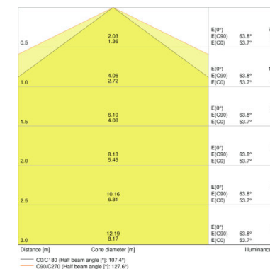
DAMP PROOF LED COMPACT 1500 55 W/6500 K GR IP65
