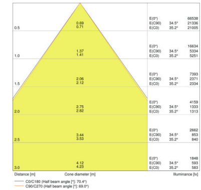
HIGH BAY LED 200 W 4000 K BK
