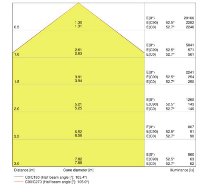
HIGH BAY LED 95 W 4000 K BK 110DEG
